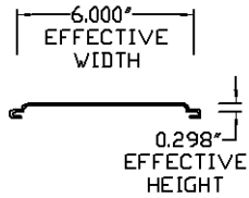
R577 ROOF DECK UPPER PIECE 6.000" X 0.298" X 0.078" EXTRUDED ALUMINUM
