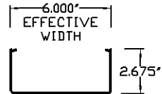
R576 ROOF DECK LOWER PIECE 6.000" X 2.675" X 0.078" EXTRUDED ALUMINUM
